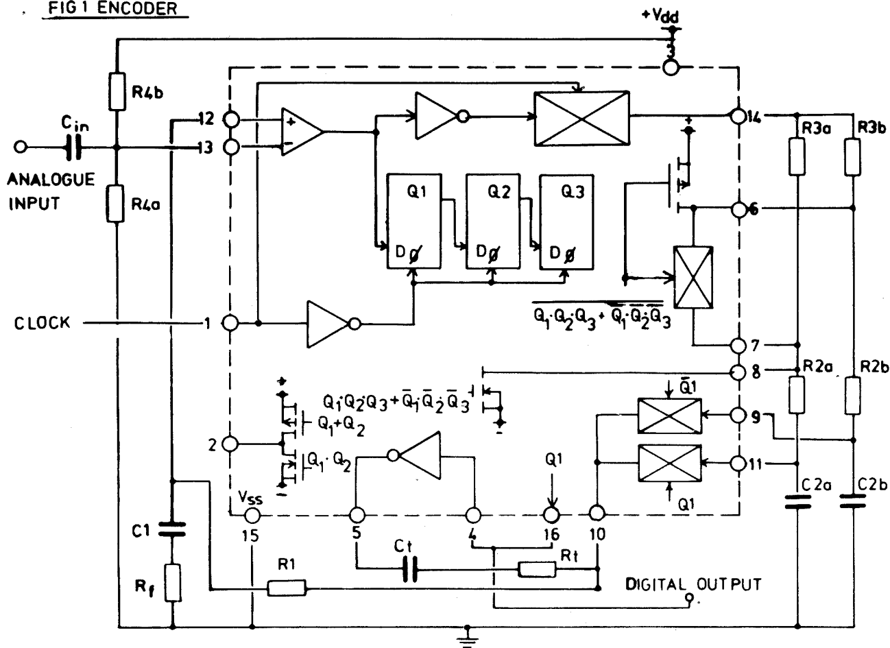
FIG 1 ENCODER
