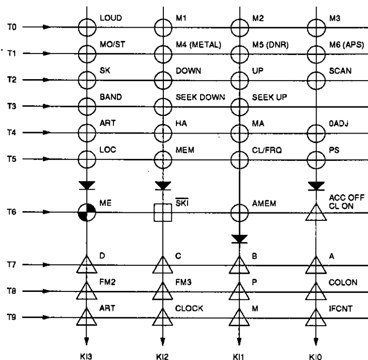
Figure 6. Keypad matrix
