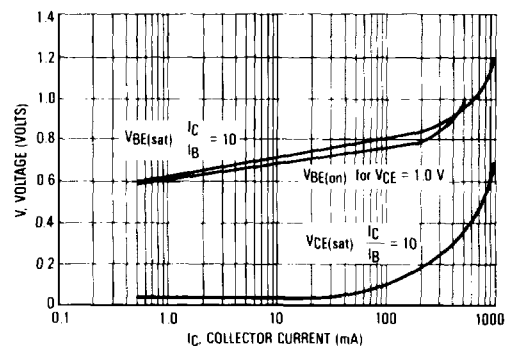
"ON" VOLTAGES
