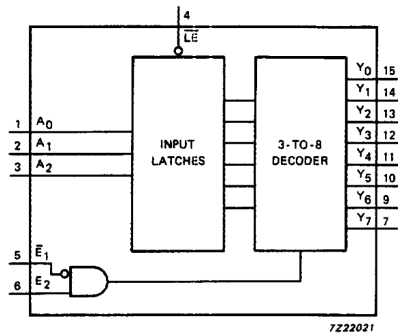
Fig.4 Functional diagram.
