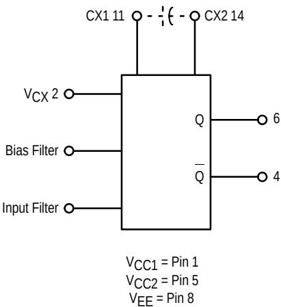
LOGIC DIAGRAM
