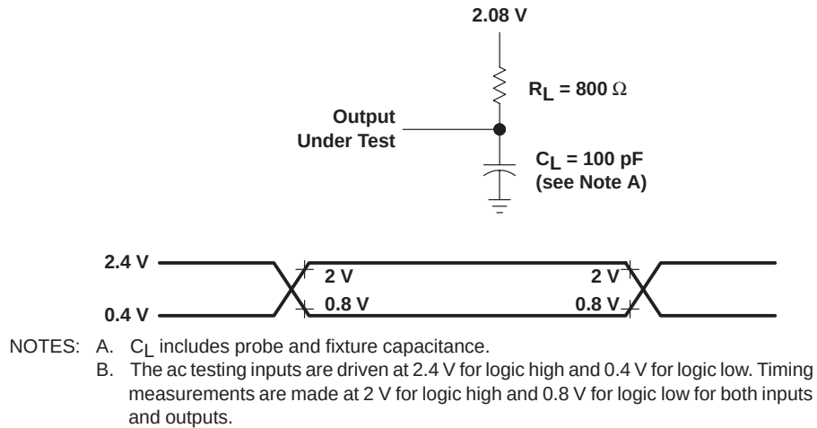
Figure 2. AC Testing Output Load Circuit
