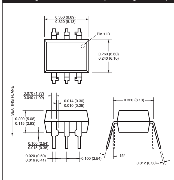
Package Dimensions (Through Hole)
