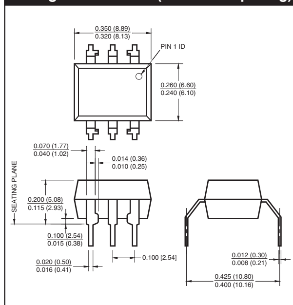
Package Dimensions (0.4" Lead Spacing)
