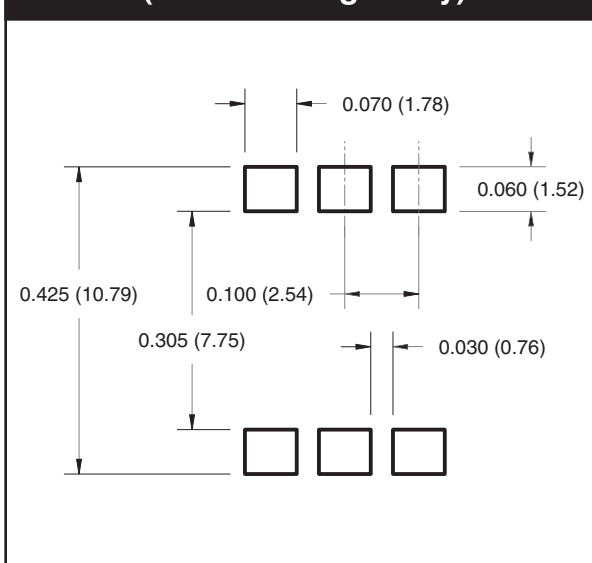
Recommended Pad Layout for Surface Mount Leadform (White Package Only)
