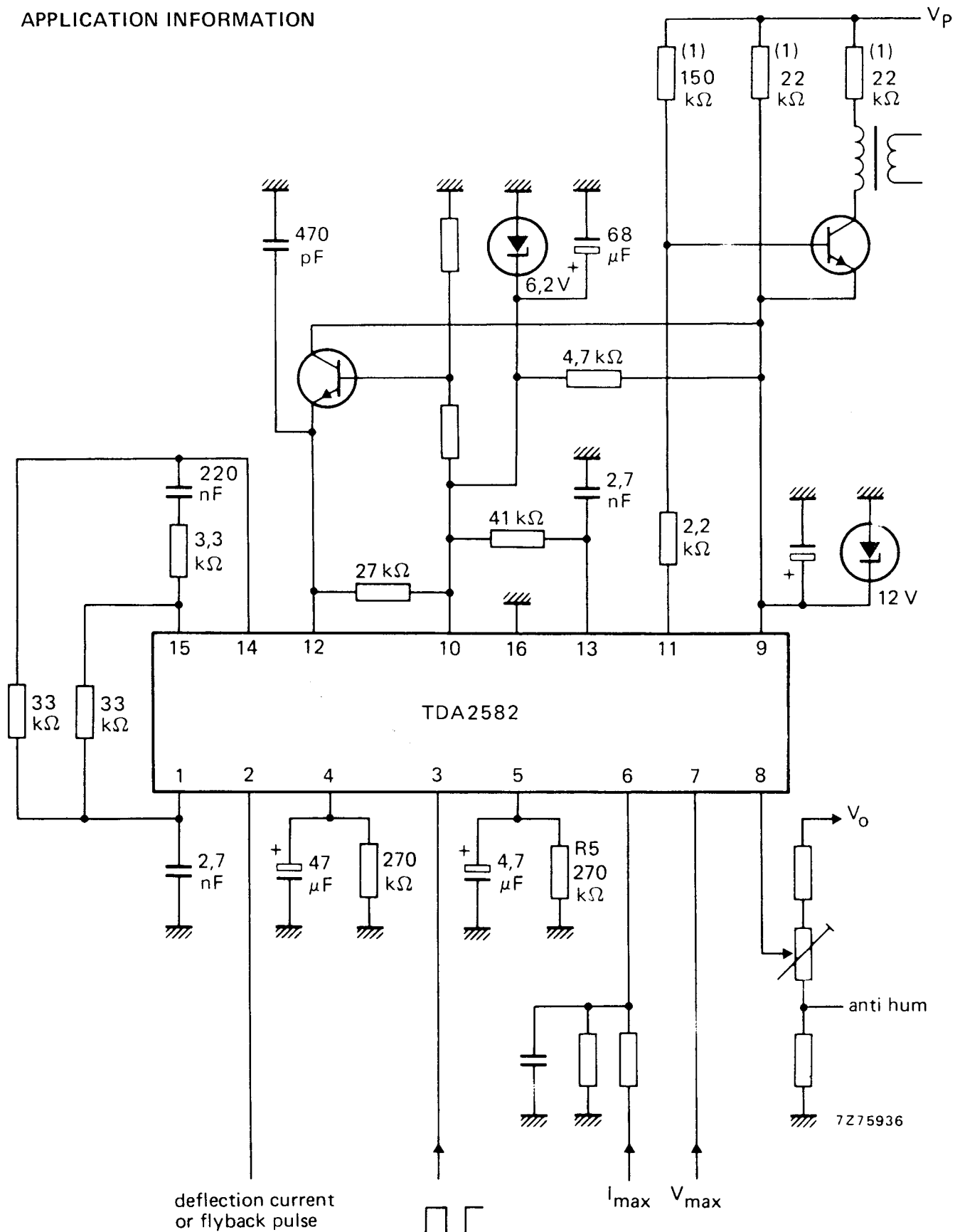
Fig. 4 Circuit diagram.
